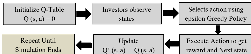
Fig. 3. Schematic Diagram of the Q-Learning ABM Model
