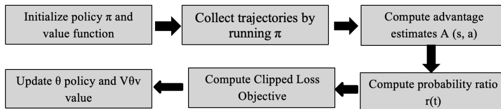
Fig. 5. PPO Model
